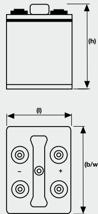
L2V470 - L2V575
